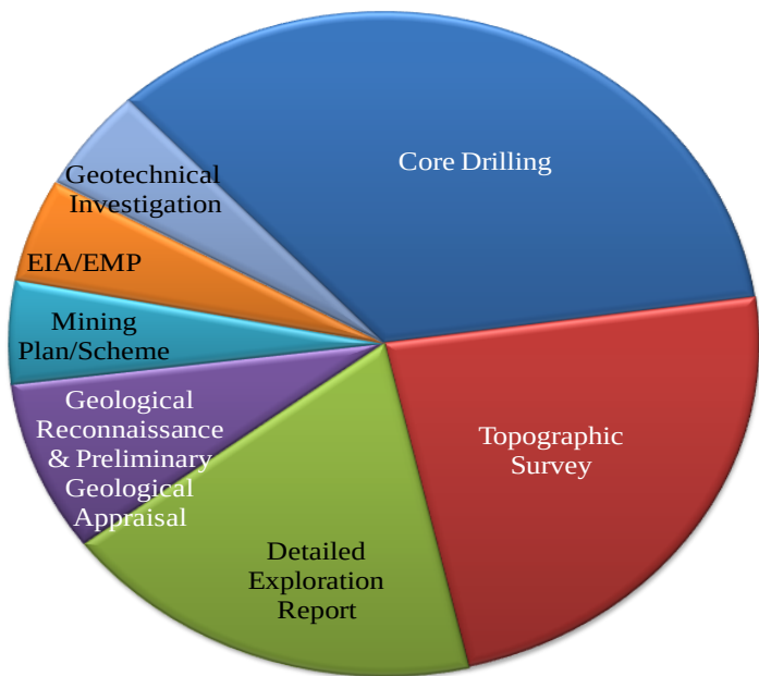
JOB CATEGORIZATION
